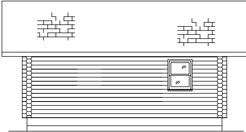
BACK ELEVATION
