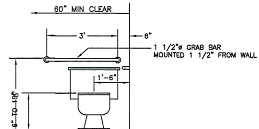
TYPICAL H.C. TOILET 1/2" = 1'-0"
